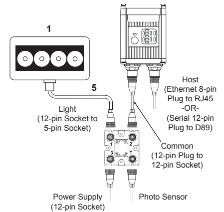
Figure E Hi-Brite Series Illuminators with QX-1 Interface Device.
