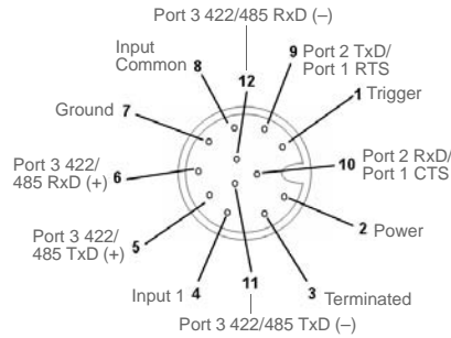
Connector B (Serial) M12 12-pin Socket
