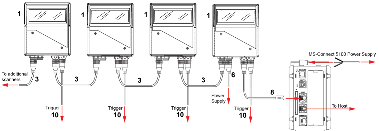
Multidrop Network with MS-Connect 5100
