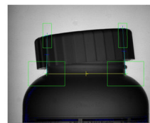
Cap Presence/Position
