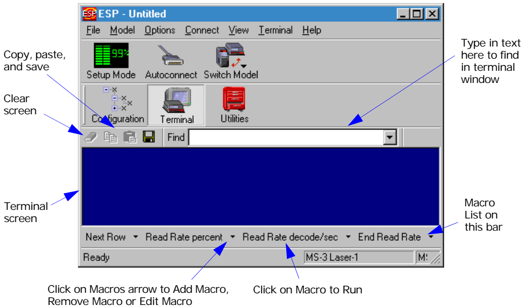
Figure 6-1 Terminal Window
